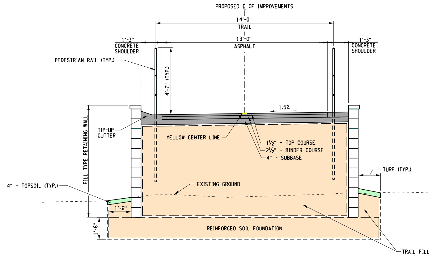
TYPICAL ASPHALT TRAIL SECTION WITH FILL TYPE RETAINING WALL
