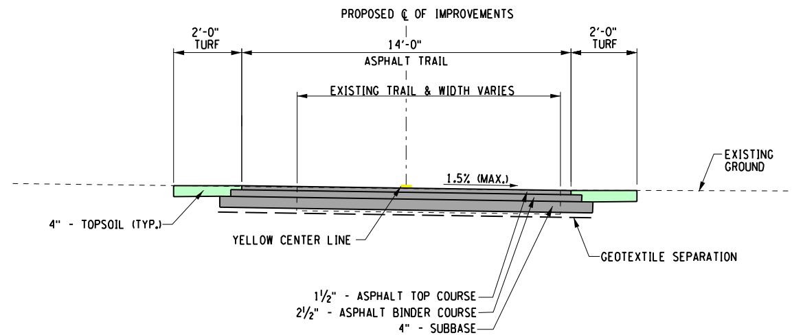
TYPICAL TRAIL SECTION (AT GRADE) FULL DEPTH RECONSTRUCTION
