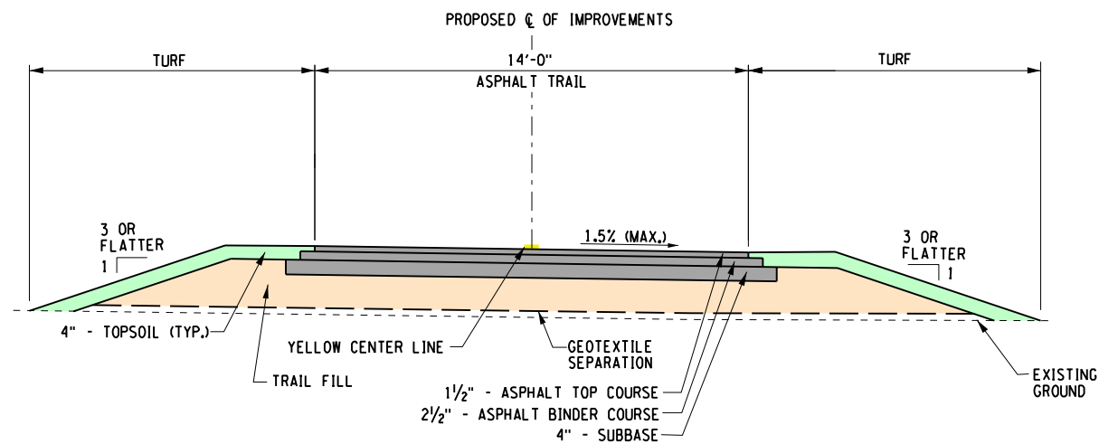
TYPICAL TRAIL SECTION (ABOVE GRADE) FULL DEPTH RECONSTRUCTION
