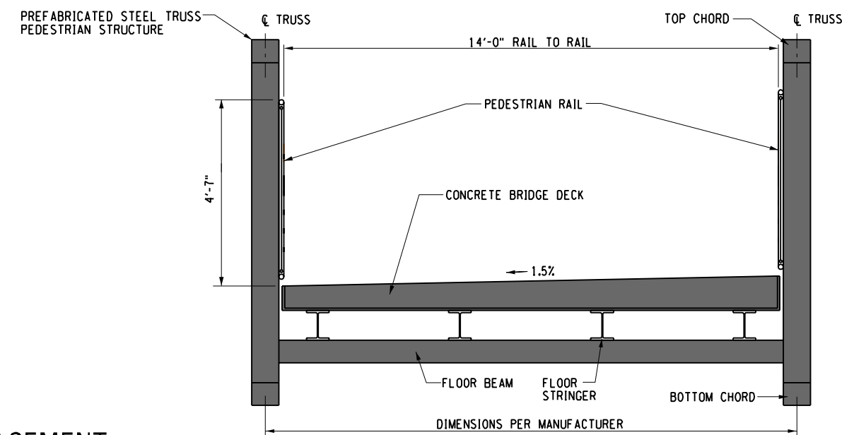
BRIDGE SECTION
